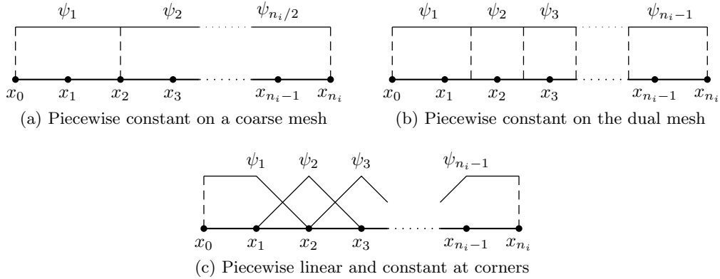
Figure 1: Possible choices for the discretization of the control
