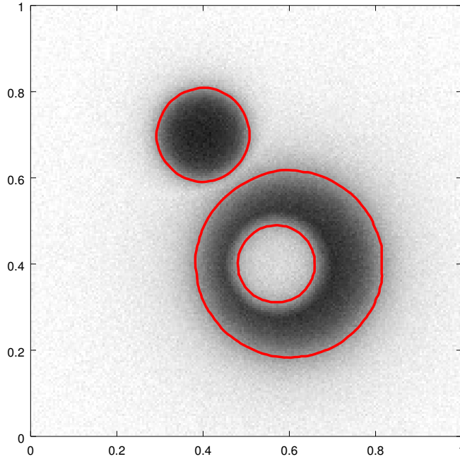
FIGURE 7. Our goal of the example optimisation problem considered for the numerical experiments in Section 5 is to find a shape matching one segment of a give grey-scale image. Here, we have not yet applied any constraints so far.
