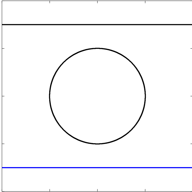
(B) Projected shape \pi(\Omega_t) .
